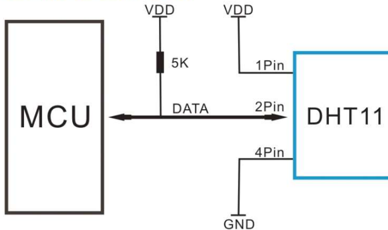
Figure 1 Typical Application
