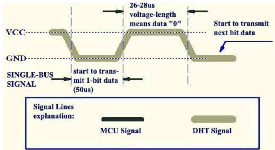
Figure 4 Data "0" Indication
